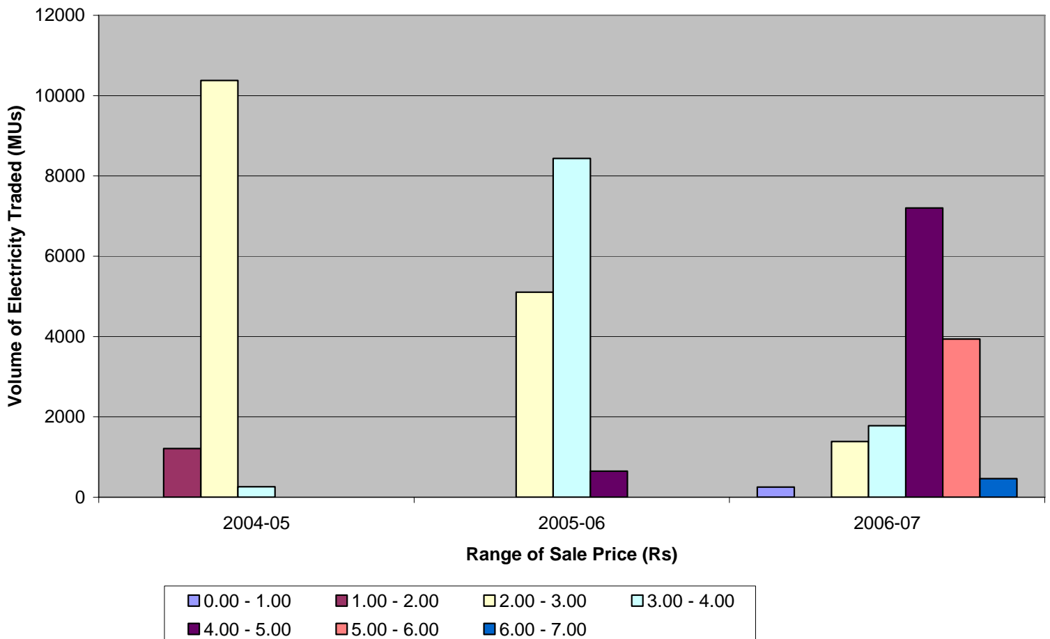
Volume of Electricity Traded by the Trading Licensees and its Sale Price
